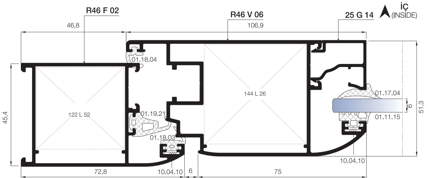
PVC AÇILIM AKSESUARINA UYGUN KANAT DETAYI VENT DETAIL FOR PVC OPENNING ACCESSORIES
