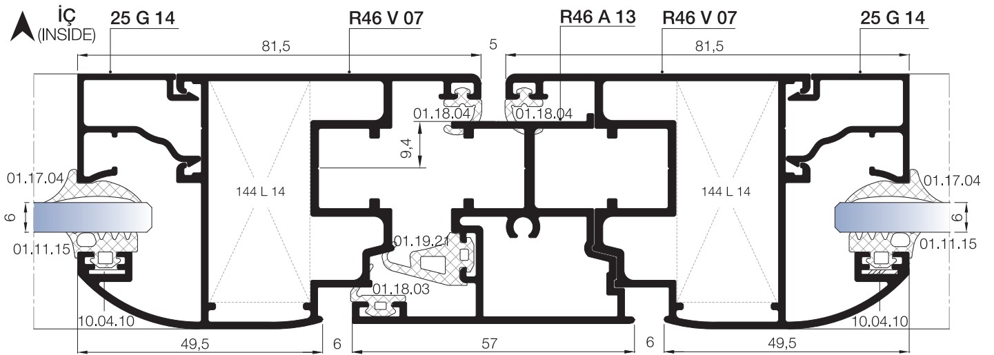
PVC AÇILIM AKSESUARINA UYGUN KANAT DETAYI VENT DETAIL FOR PVC OPENING ACCESSORIES
